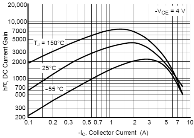
Fig. 1 DC Current Gain vs. Collector Current
